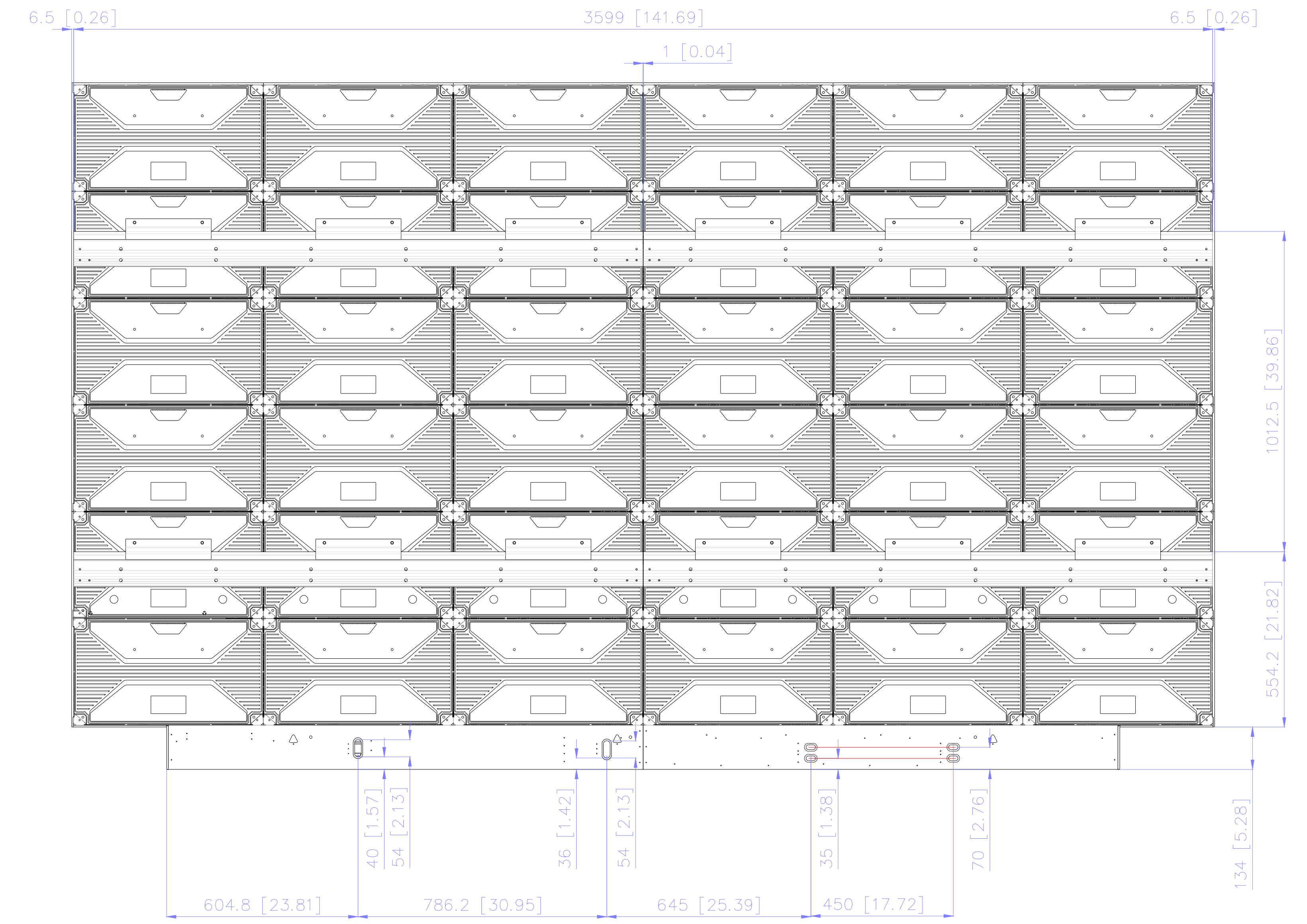
Rear View
